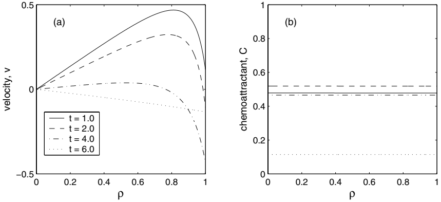
Fig. 4. Controlled granuloma growth: Graph showing the spatial distribution of (a) the internal velocity, v , and (b) the chemoattractant, C , at different time points with \psi = 500 , \beta_0 = 100 and \lambda = 100 , other parameters are as in Table 1.
