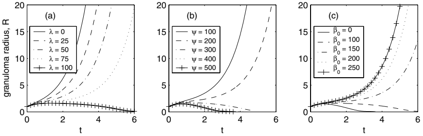
Fig. 1. Graph showing how the granuloma radius, R , varies with time, t , for: (a) \psi = 500 , \beta_0 = 100 and \lambda is varied; (b) \beta_0 = 100 , \lambda = 100 and \psi is varied (c) \psi = 500 , \lambda = 100 and \beta_0 is varied. Other parameters are as in Table 1.
