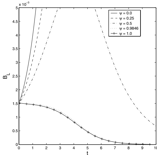
Fig. 9. Graph showing how the bacterial load, B_L , changes with time, t . The two curves that ensure that \partial_t B_L|_{t=0} \leq 0 are also shown: \psi = 0.9846 (···) and \psi = 1.0 (—+—). Parameter values are w_l = 0.01 , w_h = 0.02 and V_r = 0.1 .
